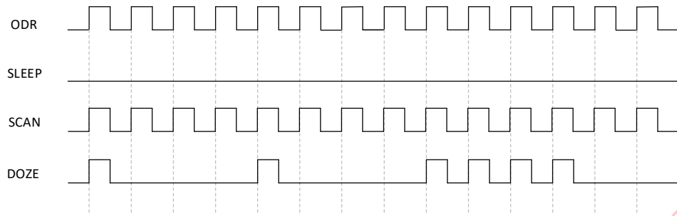
Figure3 Working modes of HX9036
