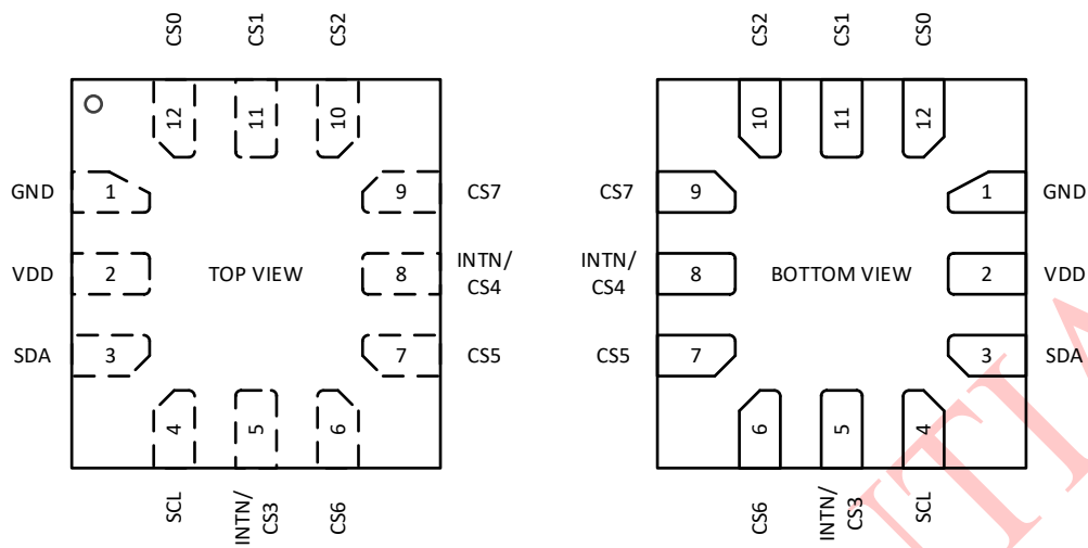
Figure1 HX9036 Pin Diagram
