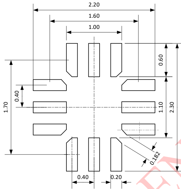
Figure13 Land Pattern
