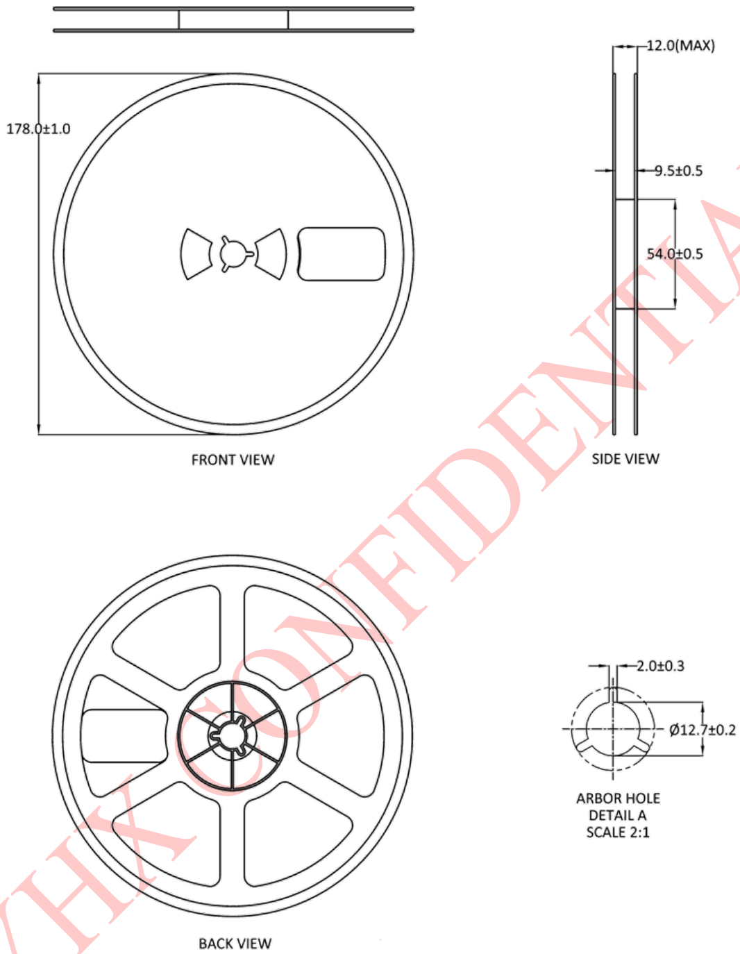
Figure12 Reel Information (Unit: mm)
