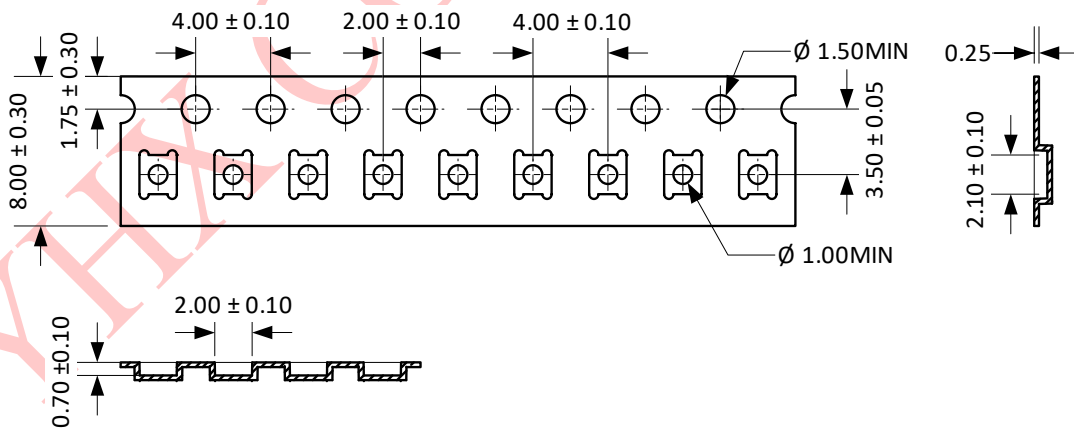
Figure11 Tape Information (Unit: mm)
