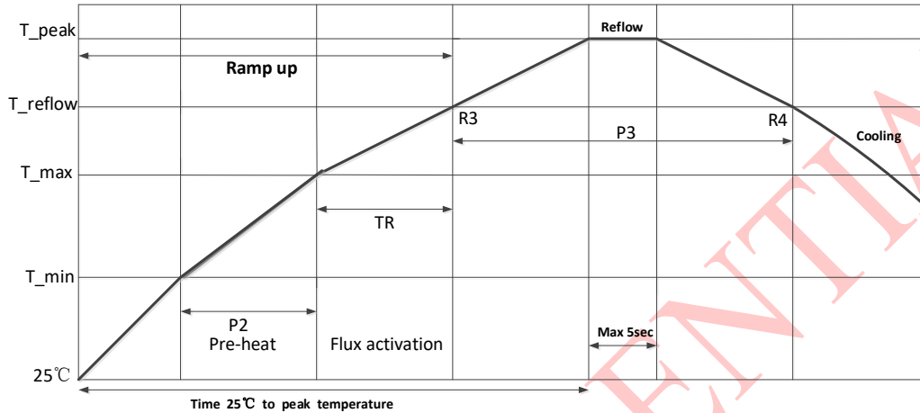
Figure11 Solder reflow profile grape
