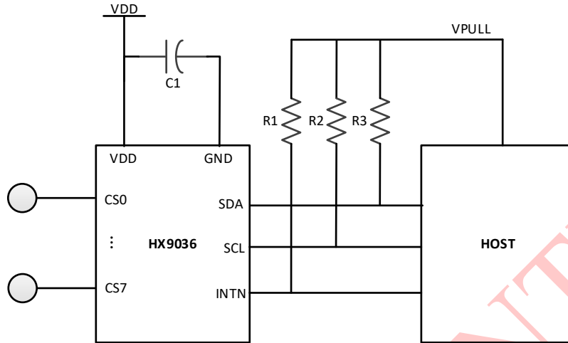
Figure9 Typical Application Schematic
