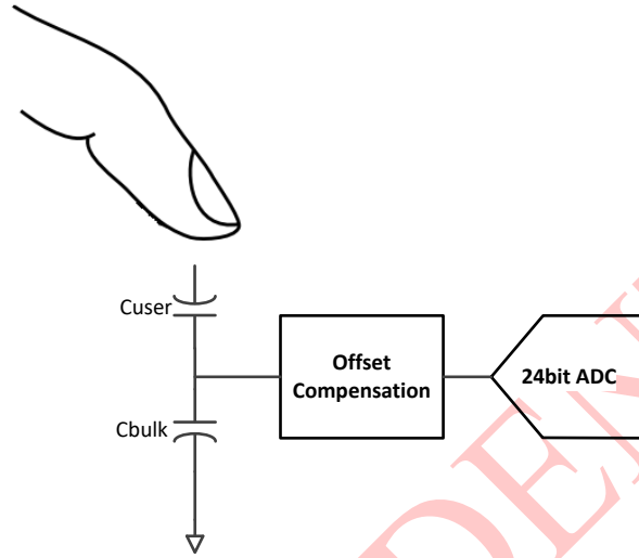
Figure5 Offset Compensation
