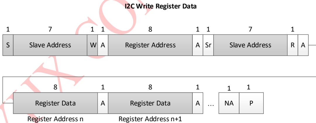
Figure7 I2C data format diagram
